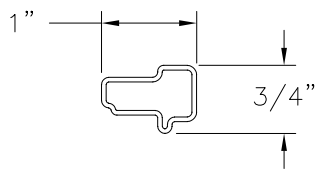
LOCK RAIL/STILE REINFORCEMENT (204A) ALUMINUM 6063-T5
