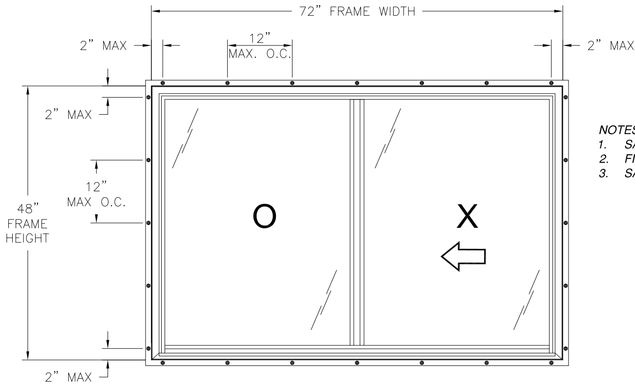
400/475 VINYL HORIZONTAL SLIDER WINDOW EXTERIOR VIEW
