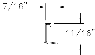
GLAZING BEAD EXTRUDED RIGID PVC
